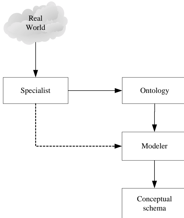
Figure 4 – Ontology-driven modeling process
